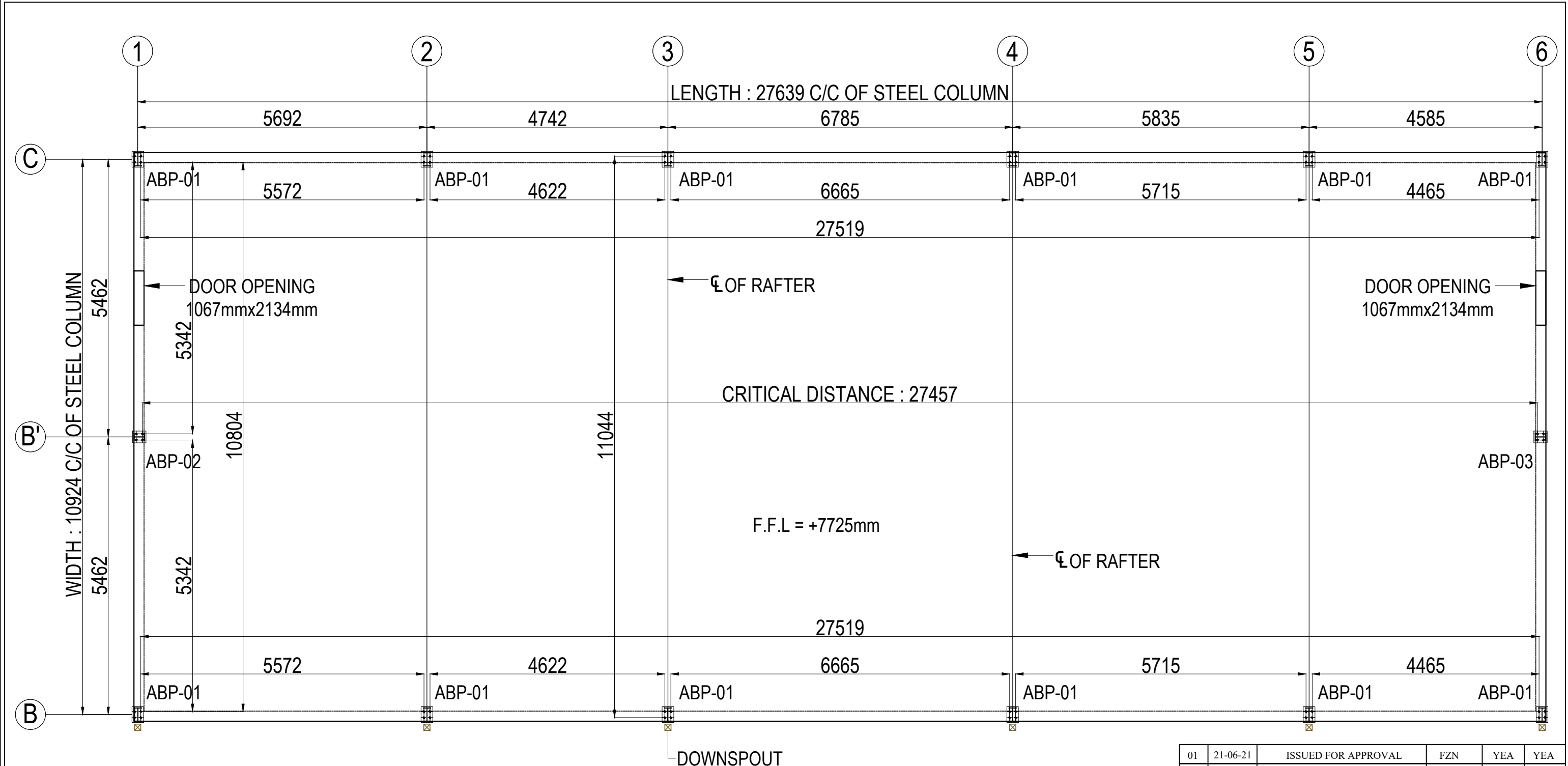
ANCHOR BOLT LAYOUT PLAN
